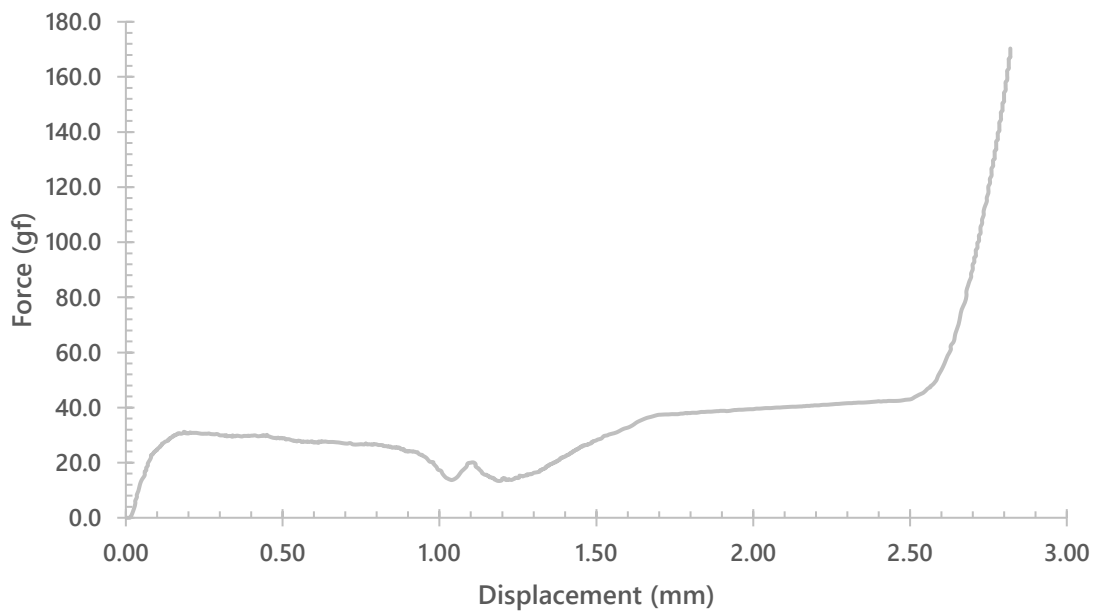
Kailh Choc Golden Kiwi White (Upstroke)
